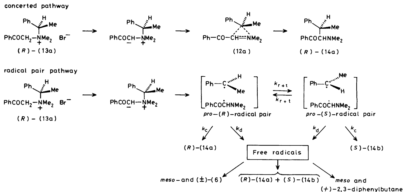
Scheme 1. Concerted and radical pair pathways for the thermal transformation of the ylide derived from the ( R )-(+)-salt (13a).
